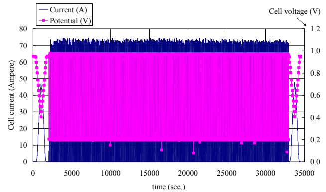
Fig. 4 Representative results of the 500 OCV-0.2V cycling. Results shown here are the data of 9501-10000 cycles
