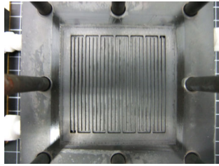
Fig. 2 MEA test fixture employed in this study has a triple channel serpentine flow field and an area of 25cm 2
