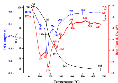
Fig. 4 Thermal analysis of \text{Cu-Mn}/\gamma\text{-Al}_2\text{O}_3 (1:5). Active component content 21.0%
