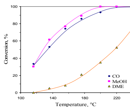
Fig. 12 Temperature dependence of CO, CH 3 OH and DME conversion over Cu-Mn/γ-Al 2 O 3 catalyst with Cu/Mn molar ratio 2:1
