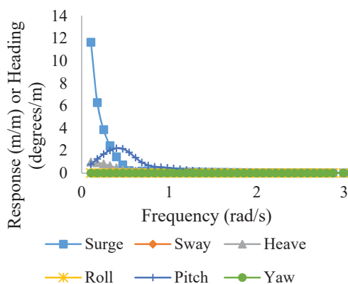
Fig. 5 Response Amplitude Operator for 0° wave heading
