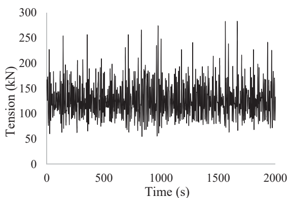
Fig. 21 Time series of mooring line 8
