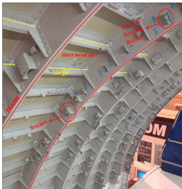
Fig. 1 An aircraft upper shell examined for assembly inspection
