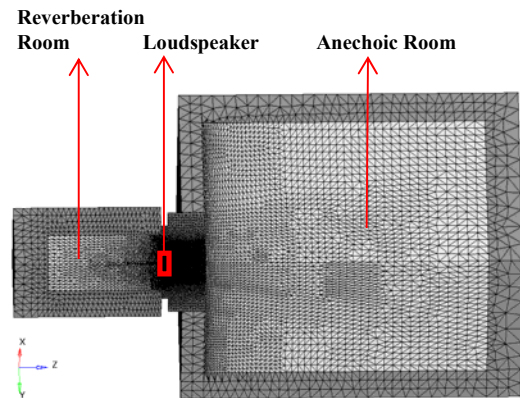
Fig. 14 Analytical model
