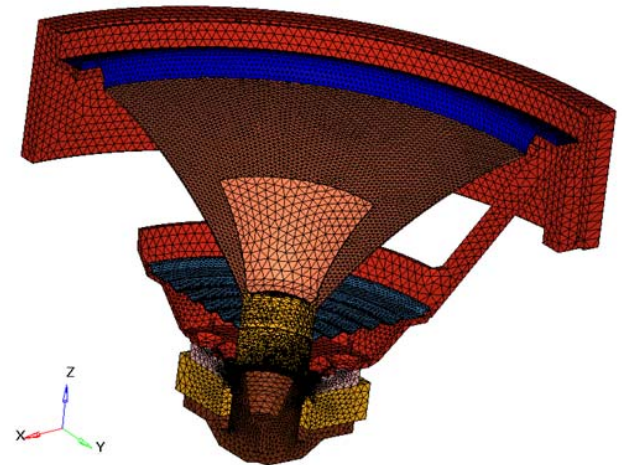
Fig. 13 Loudspeaker mesh
