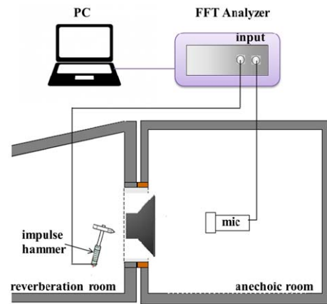
Fig. 7 Measurement system
