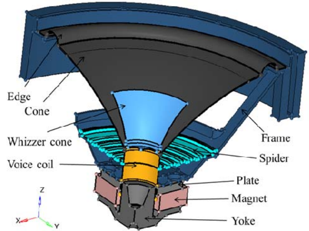
Fig. 12 1/4 solid model of a loudspeaker
