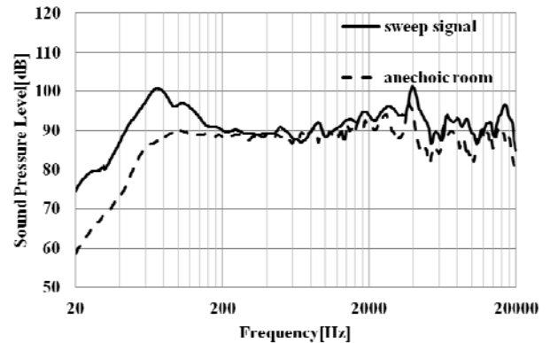
Fig. 10 Comparison of measurements in a small anechoic room and an anechoic room
