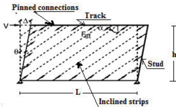
Fig. 2 Strip model
