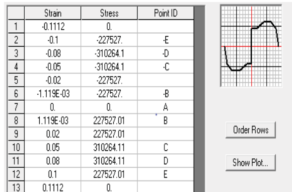
Fig. 3 Strain-Stress curve
