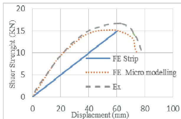
Fig. 7 Shear-displacement curve of SWP-CFS under control displacement
