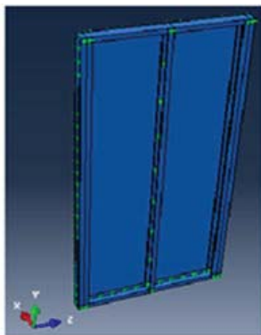
Fig. 5 Finite element model (Micro modeling)
