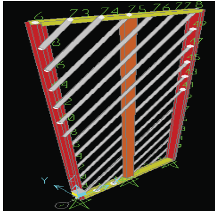
Fig. 4 FE Strip model
