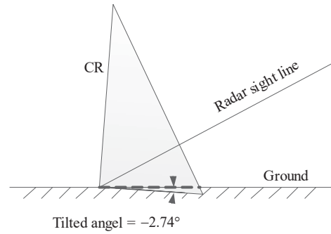
Fig. 6 Illustration of the CR deployment
