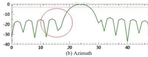
Fig. 11 Range and azimuth 1-D impulse response functions of a hexagonal trihedral CR
