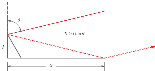
Fig. 4 Geometry of the bottom-extended trihedral CR
