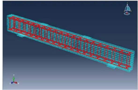
Fig. 4 Reinforcement of Beam in ABAQUS
