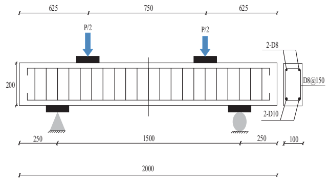
Fig. 2 Details of Geopolymer Concrete Beam
