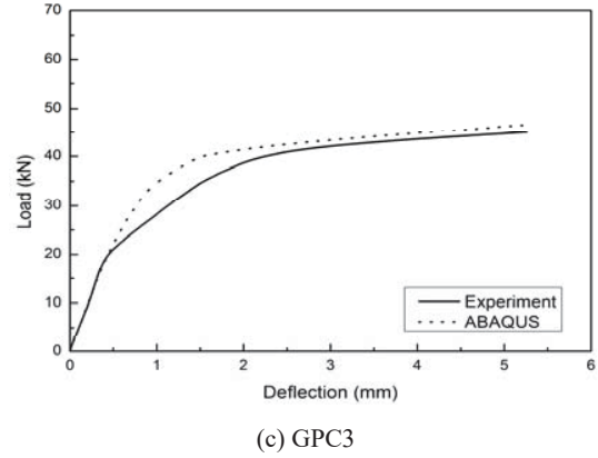
Fig. 7 Load Deflection Curve of the Geopolymer Concrete Beam
