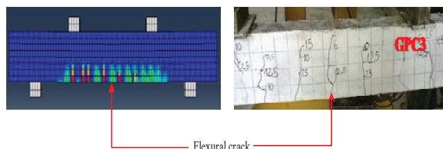
(c) Crack Patterns of mixture GPC3
