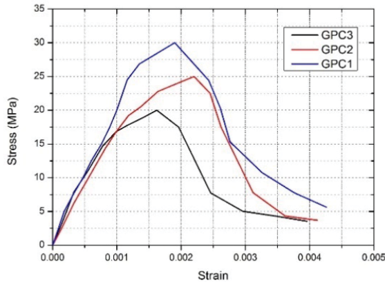
Fig. 6 Uniaxial Compression Test of Concrete
