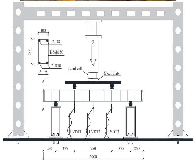
Fig. 3 Schematic of Four-Point Bending Test
