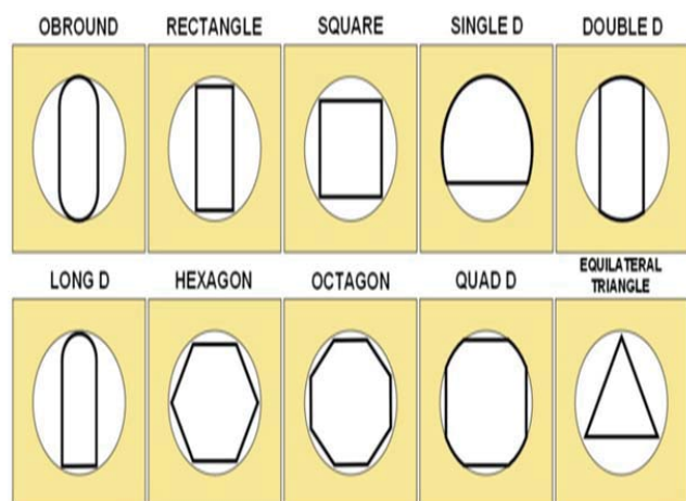
Fig. 6 Common 2-D Punch Shapes (Courtesy Unipunch™)
