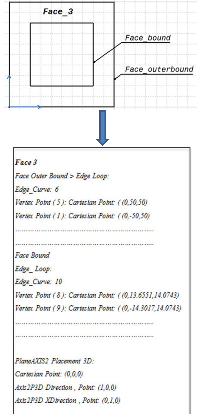
Fig. 3 Face_outerbound and Face_bound loops
