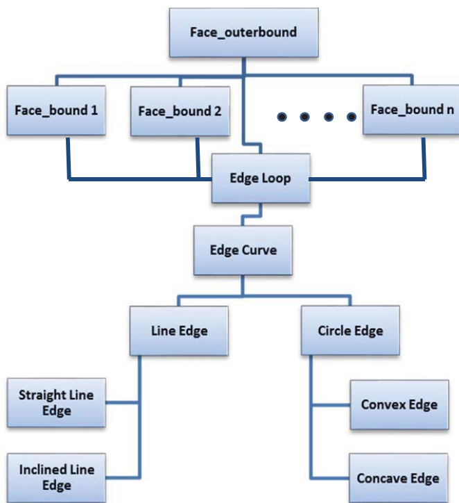
Fig. 4 Face-Loop-Edge Hierarchy
