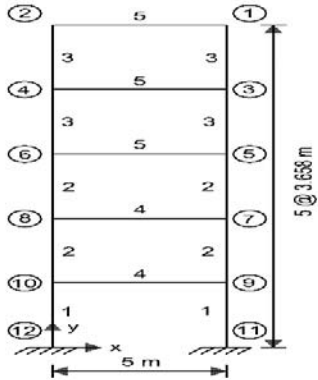
Fig. 6 A Five-story bending frame
