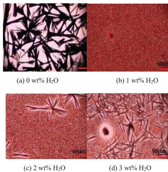
Fig. 3 Optical images of perovskite films consisting of various amounts of DI-H 2 O in PbI 2 /DMF solution (DI-H 2 O content is wt% ratio vs DMF)
