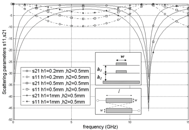
Fig. 2 Effect of height of layers on frequency response of two parallel coupled lines
