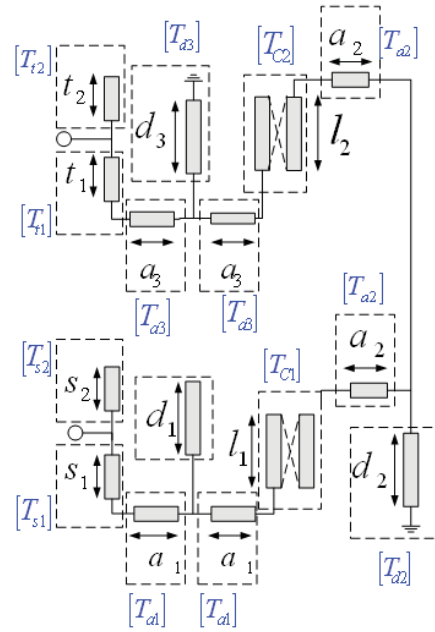
Fig. 4 The equivalent circuit of proposed multilayer microstrip filter
