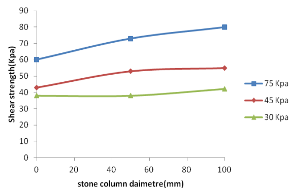
Fig. 8 Shear strength mobilized at 40 mm shear displacement versus stone diameter in the case of OSCs
