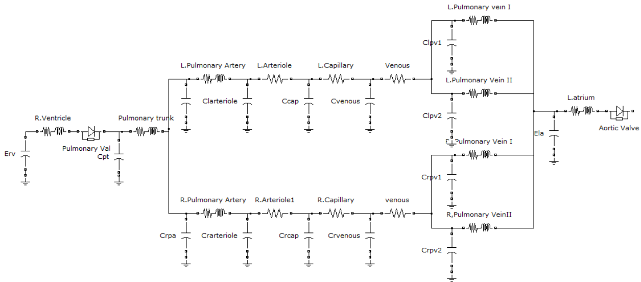
Fig. 4 Lumped Parameter Model for Pulmonary Circulation
