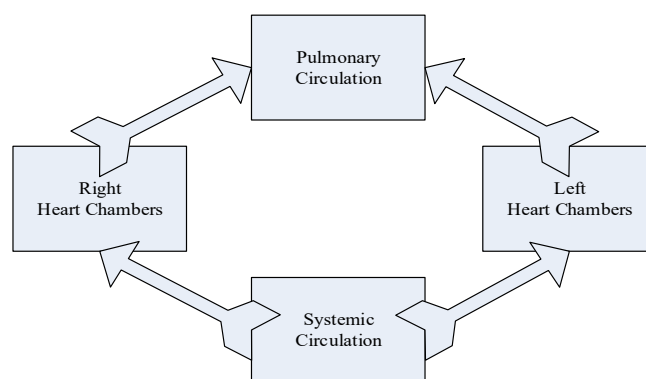
Fig. 1 Hemodynamics of Cardiovascular System
