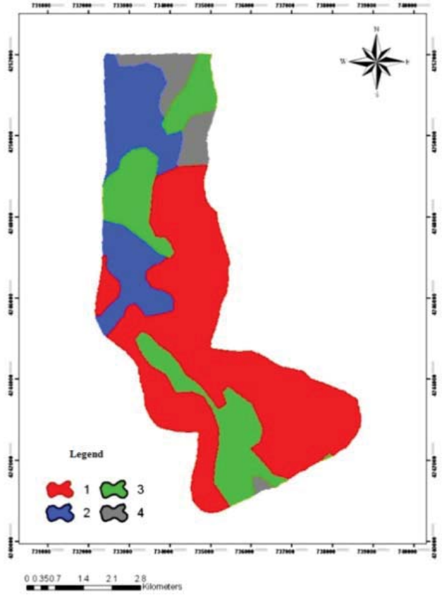
Fig. 9 The standardized map of lithology
