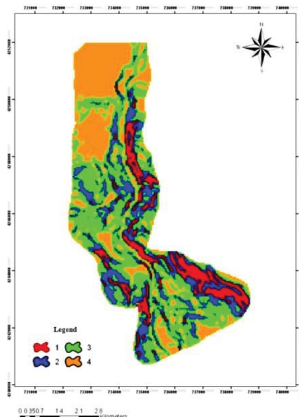
Fig. 6 The standardized map of slope
