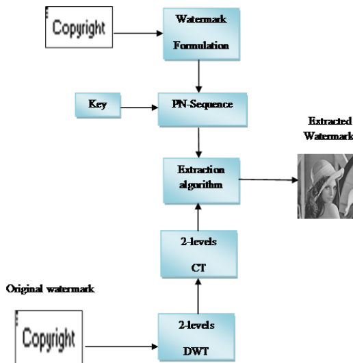
Fig. 3 DWT-CT Watermark extraction block diagram [1]
