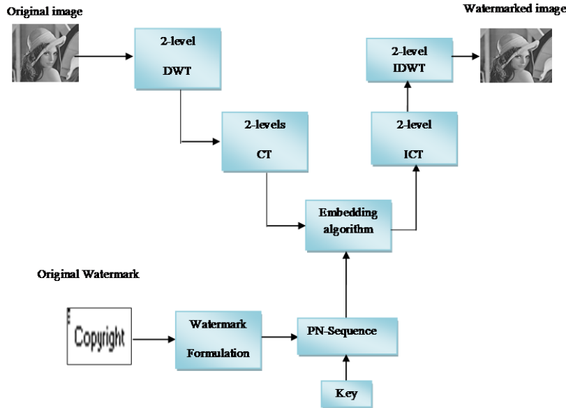
Fig. 2 DWT-CT Watermark embedding block diagram [1]
