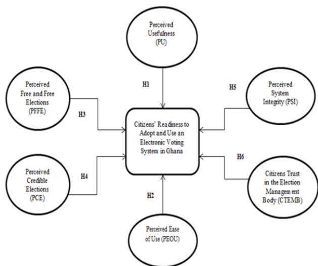
Fig. 1 Research Model [10]
