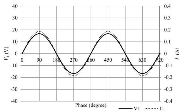
(a) I_1 and V_1 (Input waveforms)
