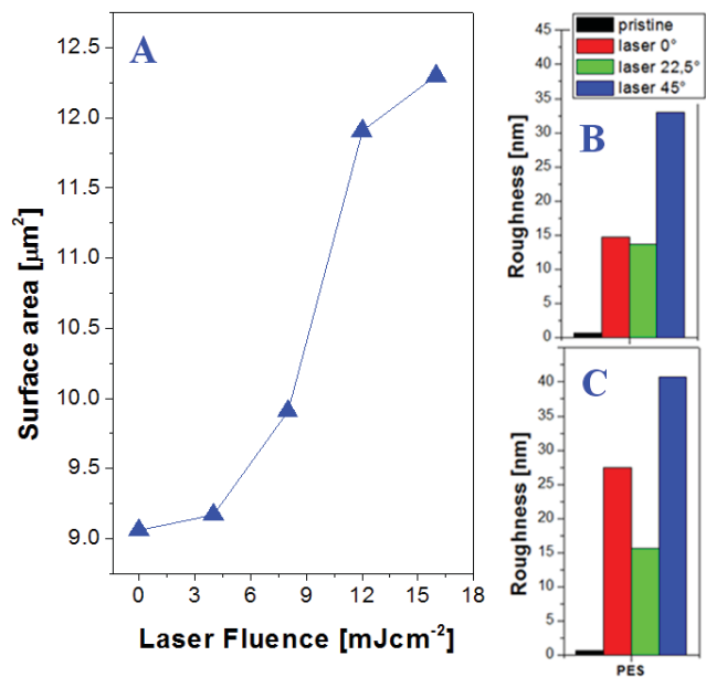
Fig. 2 The dependence of the surface area of laser-treated PES (6,000 pulses) on laser fluence (A), the dependence of PES roughness on the angle of the stage tilt at the laser fluence of 8 \text{ mJ cm}^{-2} (B) and 16 \text{ mJ cm}^{-2} (C) is introduced
