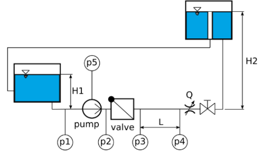
Fig. 8 Scheme of experimental stand
