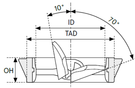
Fig. 1 Geometric parameters of mechanical heart valve [8]
