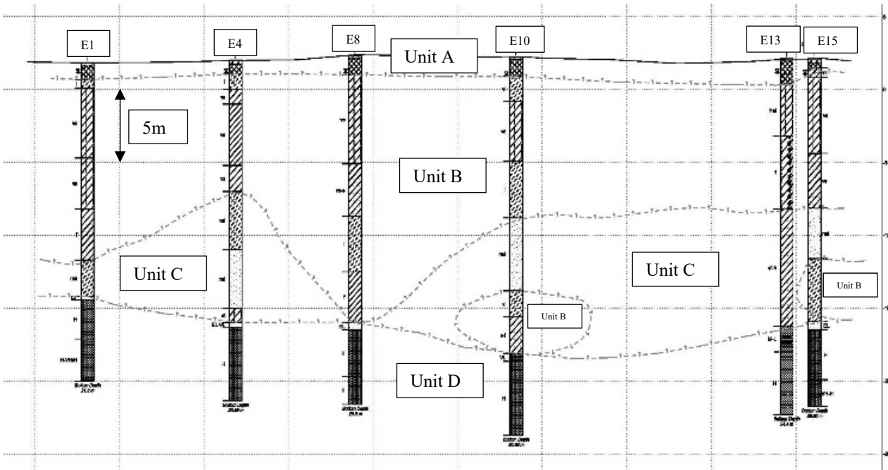
Fig. 2 Cross-section A-A'
