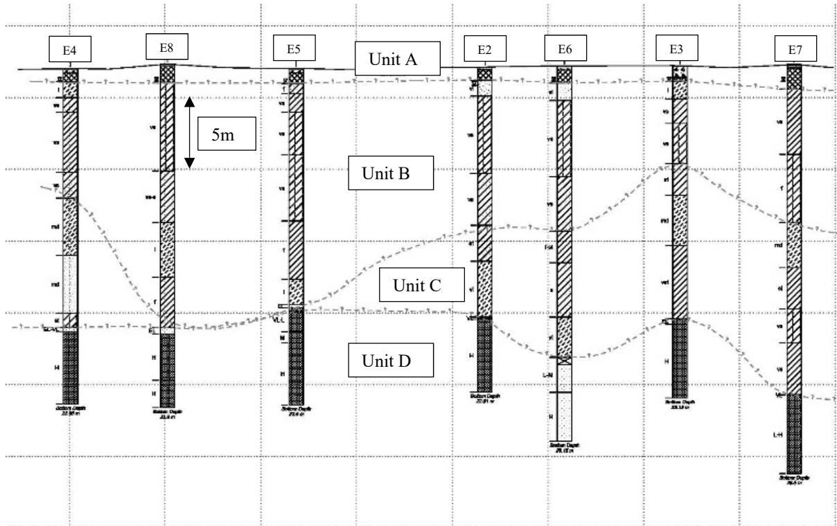
Fig. 3 Cross section B-B'
