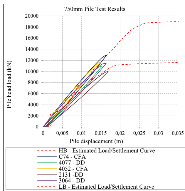
Fig. 101 750-mm estimated vs test load settlement curve
