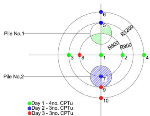
Fig. 8 Keller's CPTu test rational
