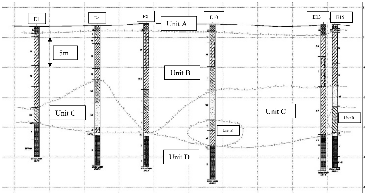
Fig. 2 Cross-section A-A'
