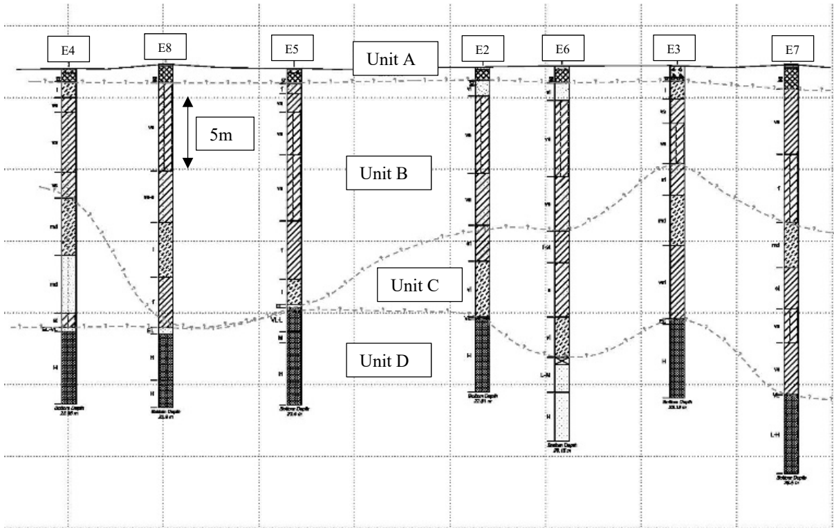
Fig. 3 Cross section B-B'
