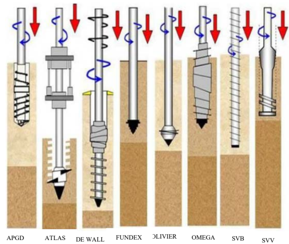
Fig. 5 Most popular full displacement augers [3]
