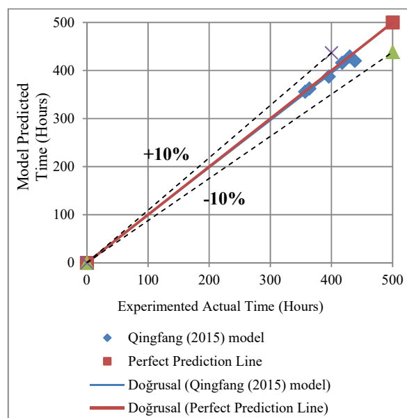
Fig. 8 Comparison of model prediction vs. actual time – column elements (two-dimensional)
