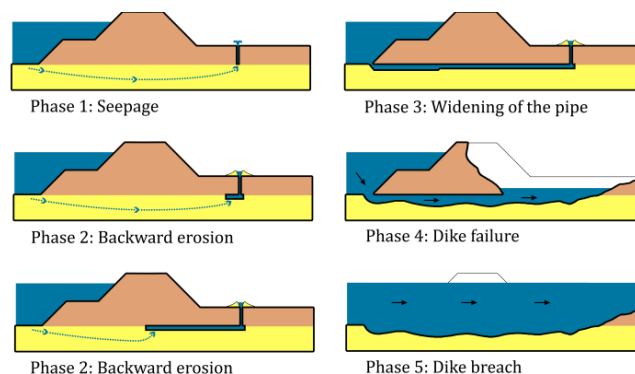
Fig. 1 Backward erosion piping [12]
