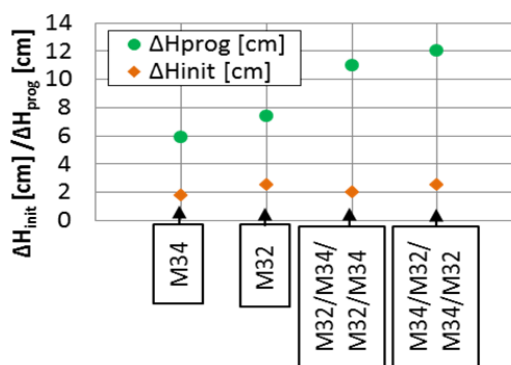
Fig. 6 Critical heads measured in the different tests
