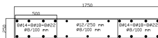
Fig. 3 Cross section of rectangular shear walls
