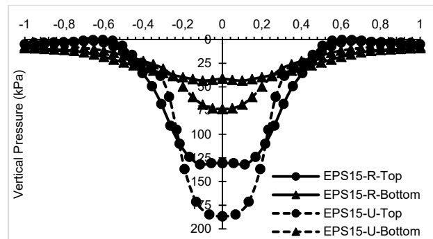
Fig. 6 Pressure distribution over and under geofoam for reinforced and unreinforced cases at 700 kPa
