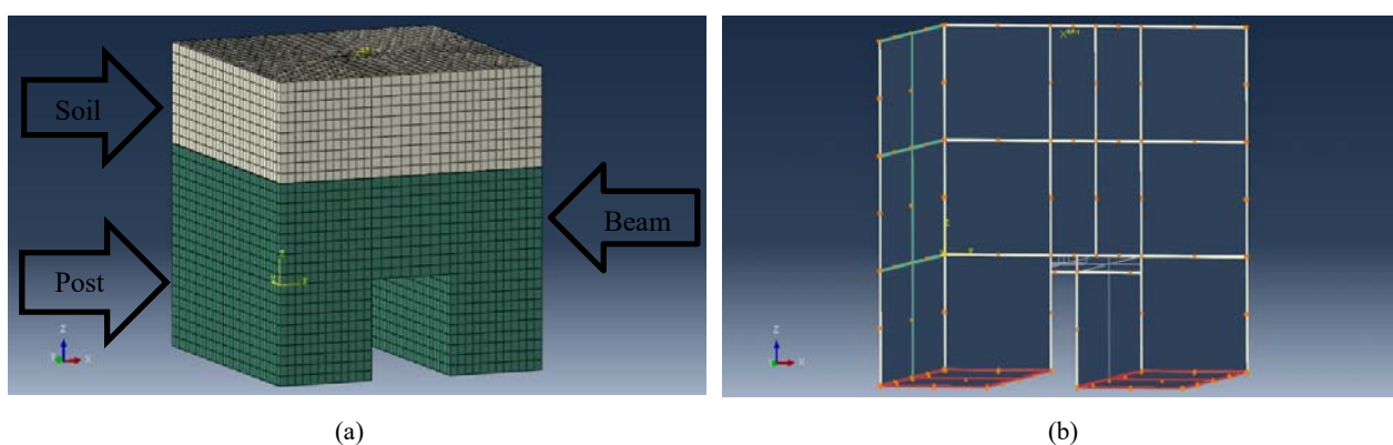
Fig. 1 3D ABAQUS model: (a) Model mesh, (b) model boundary condition
