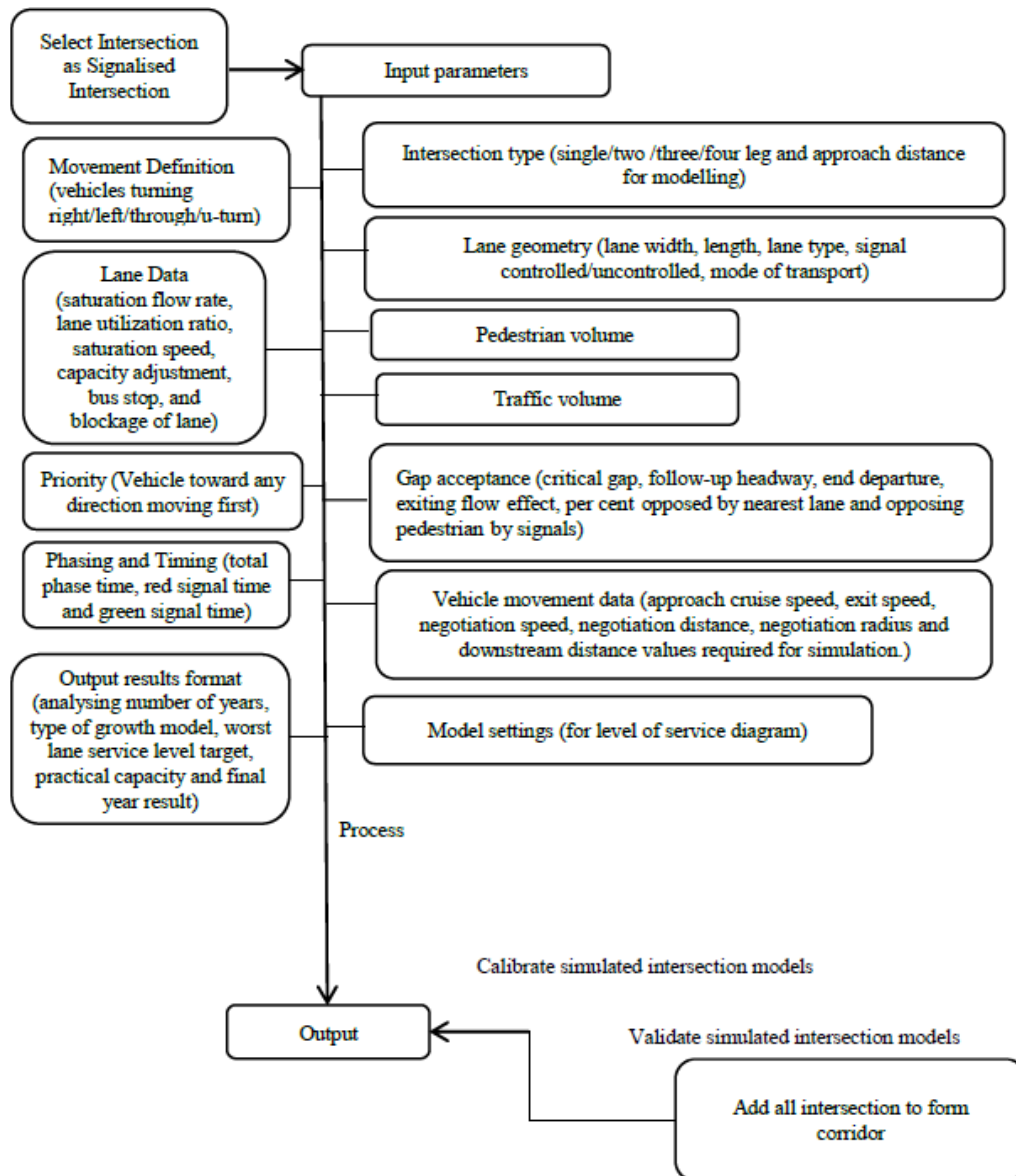
Fig. 1 Flow chart of Sidra Software
