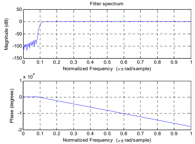
Fig. 11 The Blackman wave filter spectrogram
