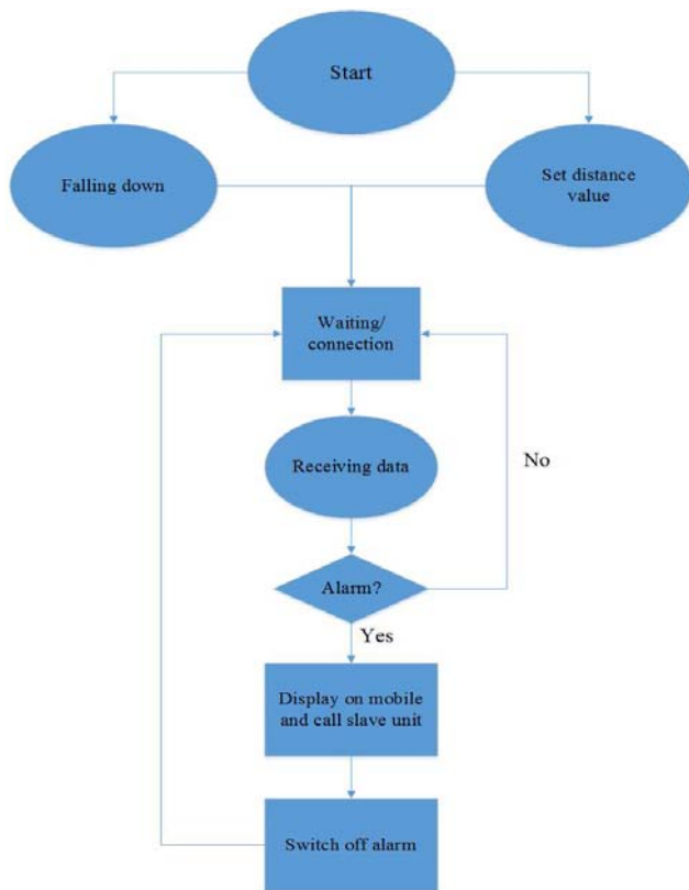
Fig. 10 Logic Flow Chart of the App
