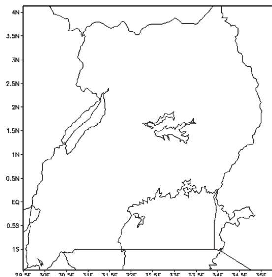
(a) The COSMO Model domain
