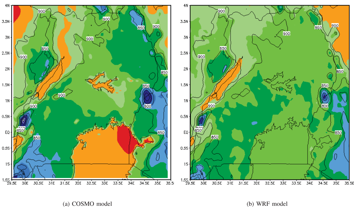
Fig. 7 Surface temperature and mean sea level pressure presented by the COSMO model (a) and the WRF model (b) on 01 st May 2013 (i.e. 01/05)
