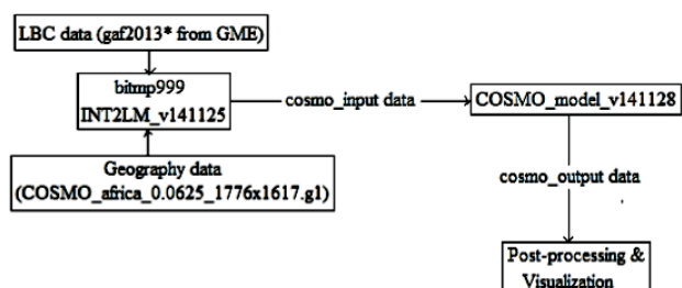
(a) The COSMO Model
