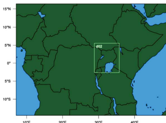
(b) The WRF Model domain
