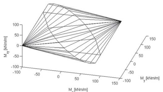
Fig. 1 Linearized Bi-Conical Nielsen's Yield Criterion
