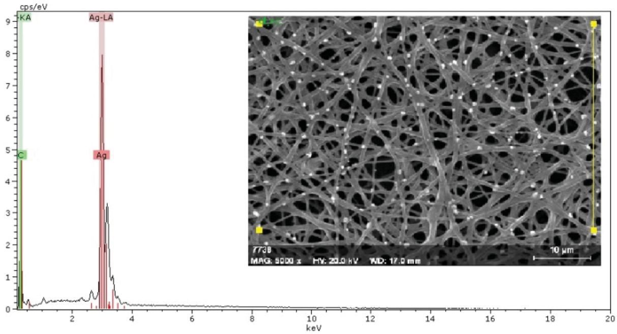
Fig. 4 SEM-EDX diagram of Ag doped CNFs
