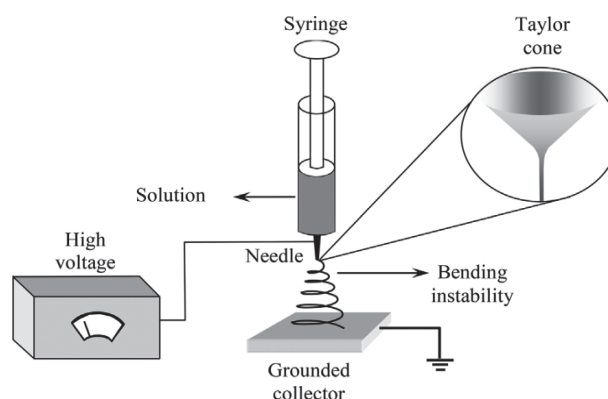
Fig. 1 Schematic diagram of the electrospinning [4]
