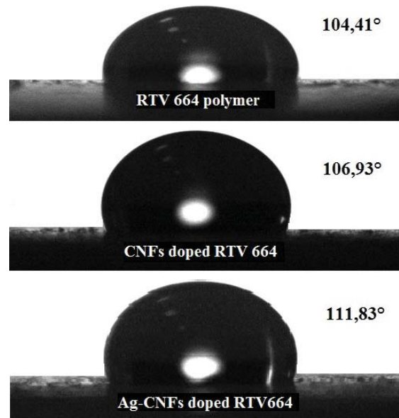
Fig. 7 Contact angles of polymer composite samples
