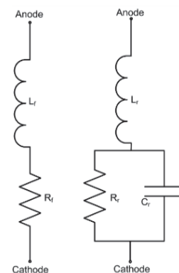
Fig. 1 Equivalent circuit of the PIN-diode (a) “ON” state (b) “OFF” state”
