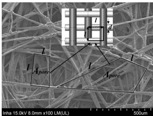
Fig. 2 A microstructure image of a commercial GDL Assumption (2) was related to the GDL's porosity. The initial porosity of the GDL p_0 , is generally defined as follows:
