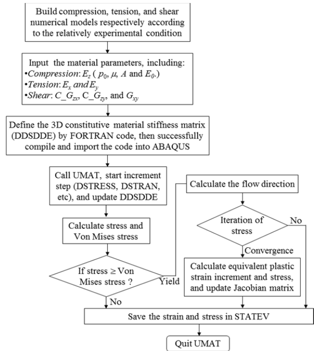
Fig. 3 The GDL's UMAT implementation flow chart
