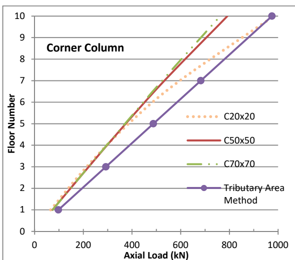
Fig. 5 Axial load for corner column
