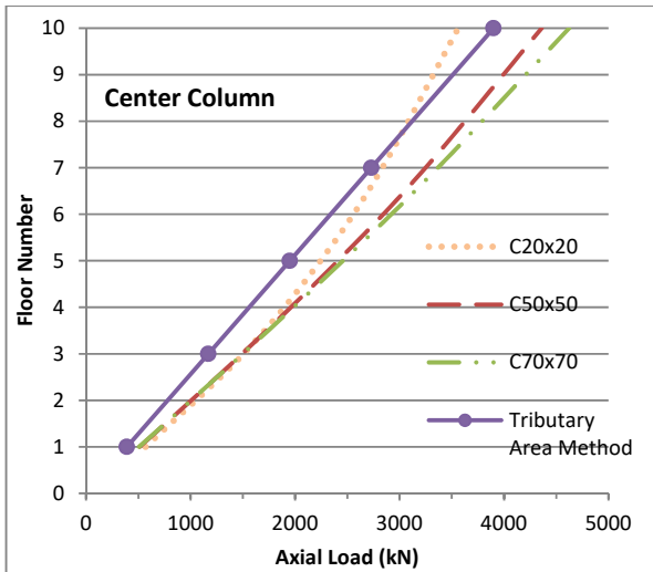
Fig. 3 Axial load for center column
