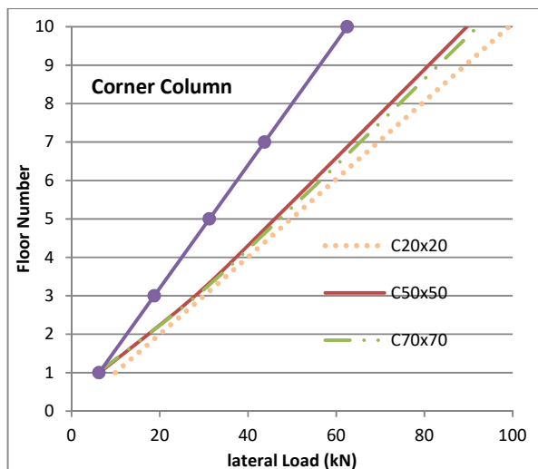
Fig. 7 Lateral load results for corner column
