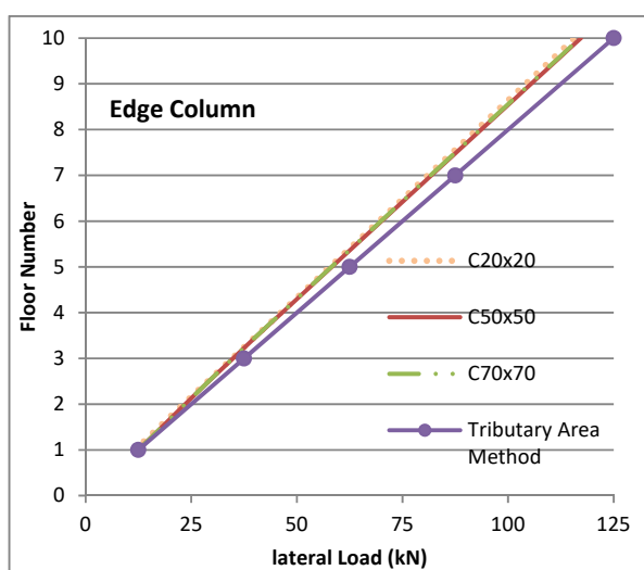
Fig. 8 Lateral load results for edge column
