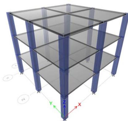
Fig. 2 General 3D model for multi-floor building
