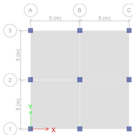
Fig. 1 Layout of the models
