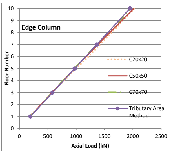
Fig. 4 Axial load for edge column
