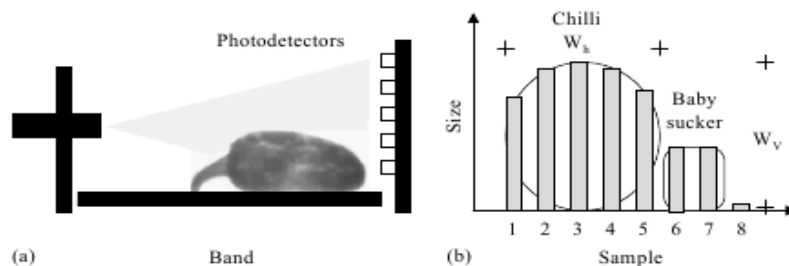
Fig. 18 Chilli size detector for grading system. (a) Laser line generator and photodetectors; (b) sampling measurements with photodetectors [70]
