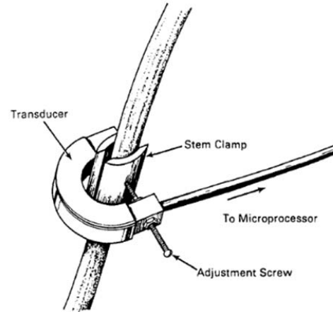
(a) Stem diameter measurement [33]
