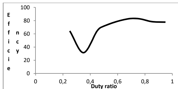
Fig. 19 (a) Graph between efficiency and duty ratio for DAB with EPS control in reverse mode at duty ratio of D_1 = 0.3 , D_2 = 0.25 to 0.95
