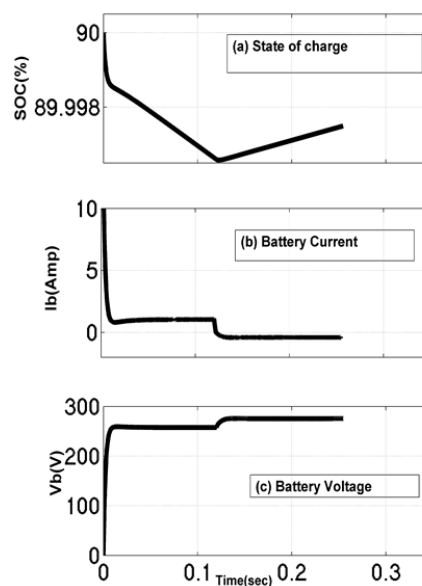
Fig. 24 Battery characteristics showing (a) State of charge of battery (b) Battery current (c) Battery voltage on HV side
