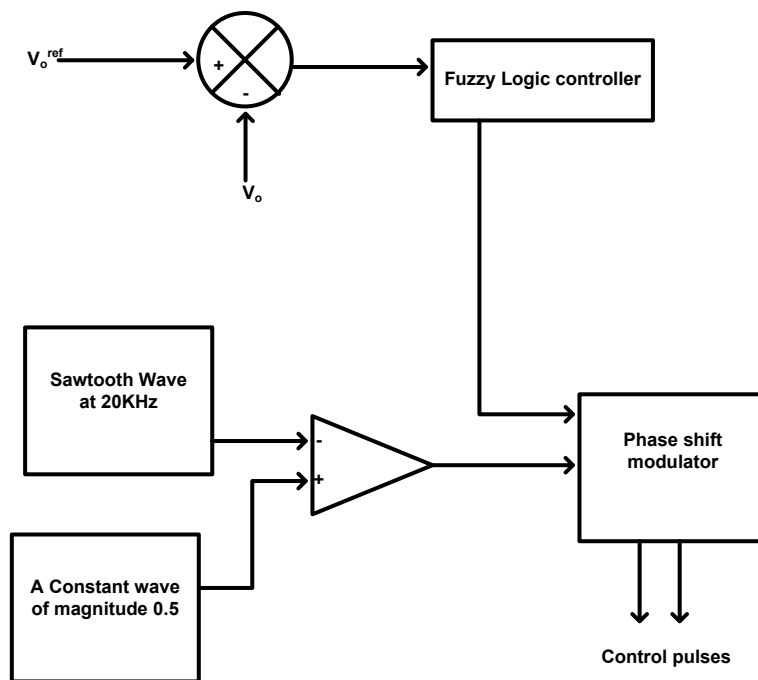
Fig. 11 Fuzzy logic based closed loop controller
