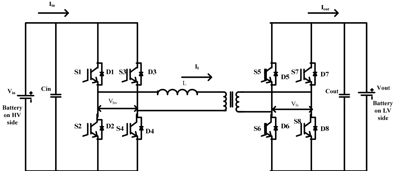
Fig.1 Power circuit diagram of single-phase DAB converter
