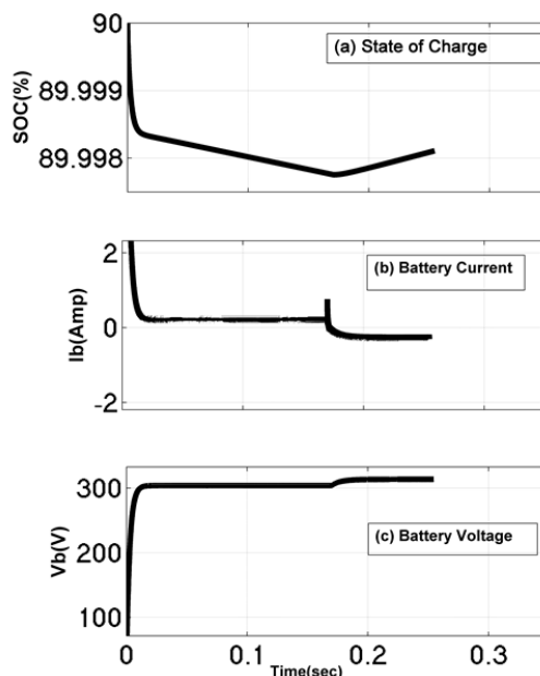
Fig. 20 Battery characteristics showing (a) State of charge of battery (b) Battery current (c) Battery voltage on HV side
