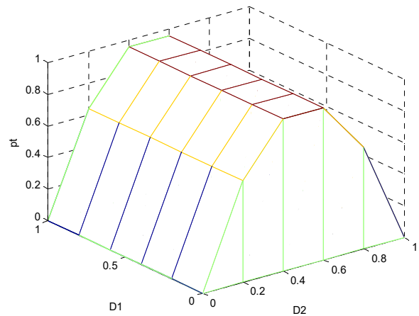
Fig. 7 Relation curve of unified transmission power with duty ratio D_1 = D_2 = D
