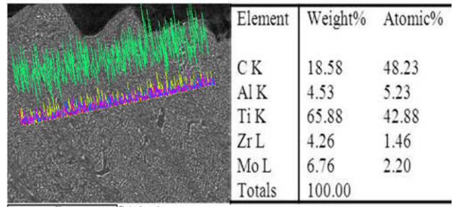
Fig. 9 Linear analyzes of a continuous chip ( a_p : 0.05 mm, v_c : 20 m/min). No changes in the local chemistry have been recorded
