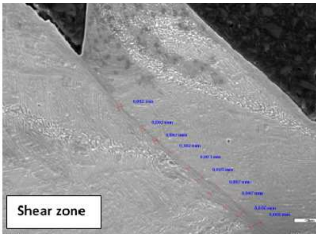
Fig. 7 Shear zone width of a Ti-6246 chip
