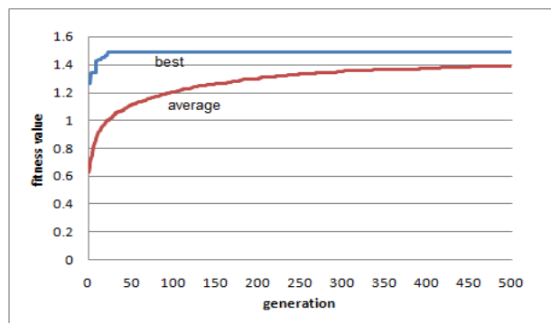
Fig. 2 The best and average fitness value
