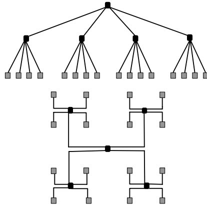
Fig. 5. MinRoot architecture
