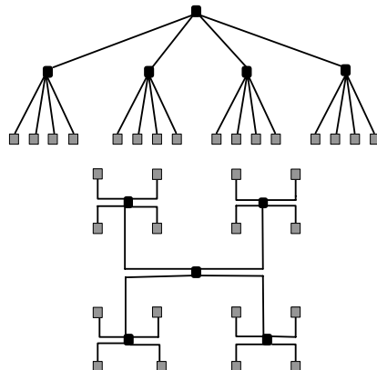
Fig. 5. MinRoot architecture
