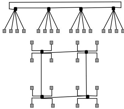
Fig. 4. CMesh architecture
