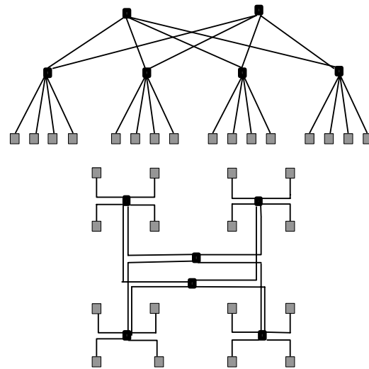
Fig. 3. BFT architecture
