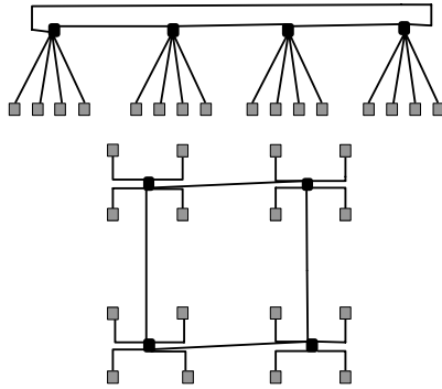
Fig. 4. CMesh architecture
