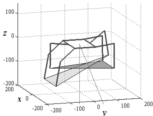
Fig. 3 Hexapod robot modeling results with fixed body plane
