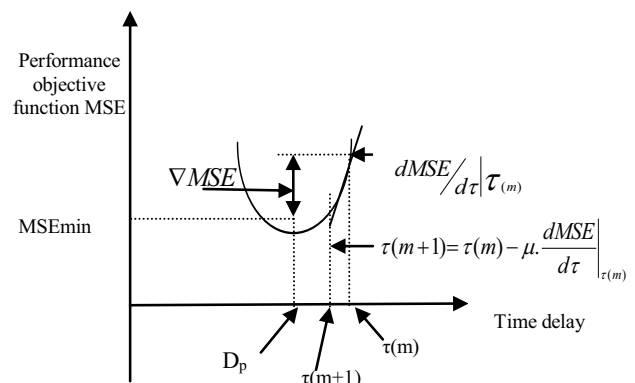
Fig. 2 Gradient descent on projection of the MSE Function
