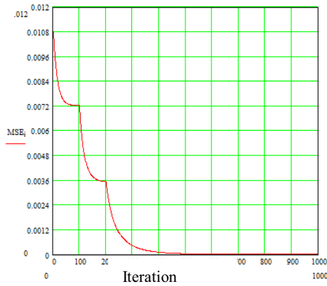
Fig. 5 Mean Square Error
