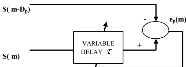
Fig. 1 Tracking time delay algorithm configuration
