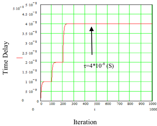
Fig. 4 Tracking Time Delay Algorithm
