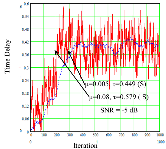
Fig. 6 The Noise and Convergence Effect on Tracking
