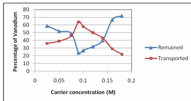
Fig. 3 Effect of carrier concentrations on transport of VO 2 + ions through SLM
