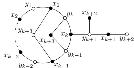
Fig. 4. y_{k+3} being adjacent to both x_1 and x_{k-1}
