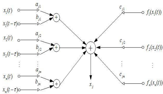
Fig. 1. Delayed Network Topology of Zero-sum Game
