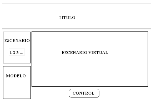
Fig. 8 Scenario structure
