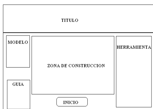
Fig. 6 User's screen
