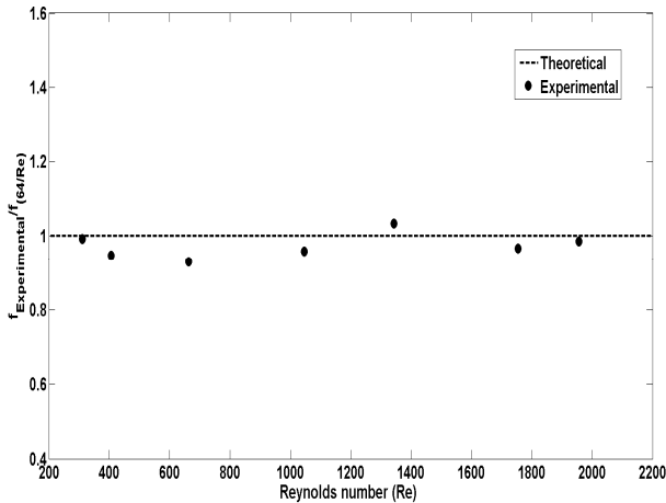
Fig. 6 Ratio of experimental friction factor to theoretical prediction for distilled water versus Re number
