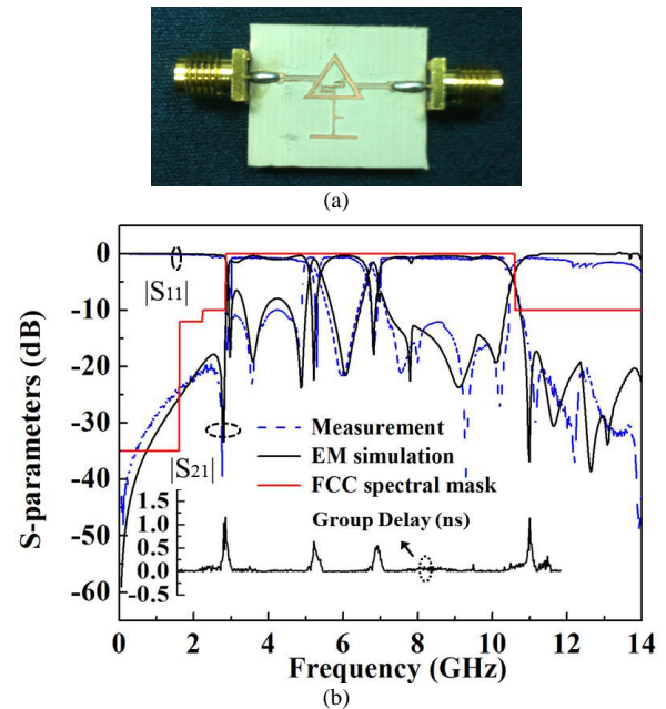
Fig. 6 (a) Photograph, (b) measured results and group delay of the fabricated UWB filter
