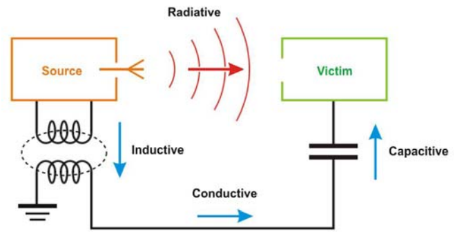
Fig. 2. EMI coupling mechanisms 1
