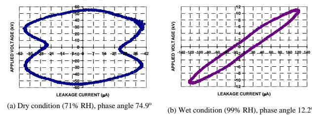
Fig. 5. Applied voltage magnitude as function of yielded LC magnitude for phase angle (a) 74.9° and (b) 12.2°
